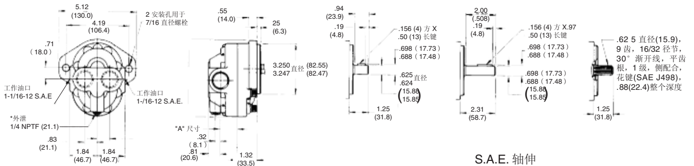
"A" 尺寸
