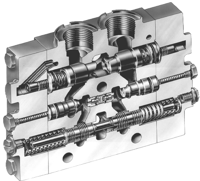
Figure 1. CMX Hydraulic Actuator Cutaway
