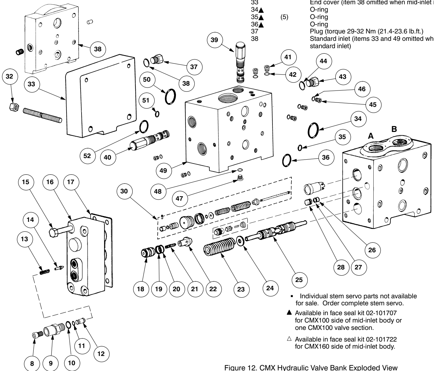
Figure 12. CMX Hydraulic Valve Bank Exploded View
