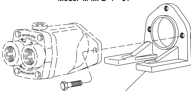
Mounting Kit FB-B-10 (Includes Screws)
